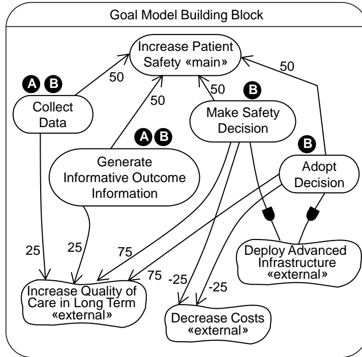
Figure 32 Goal model building block for Increase Patient Safety
