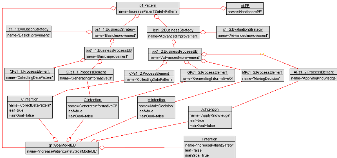
Figure 39 Object model of Increase Patient Safety pattern
