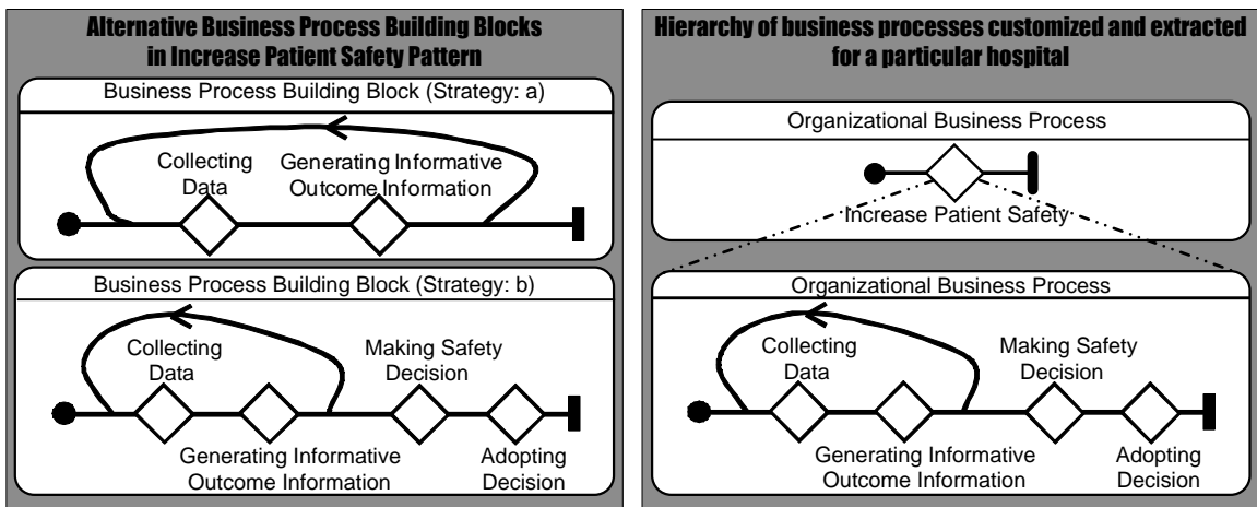
Figure 59 Using OCEM: business process building blocks, with strategy “B” being selected
