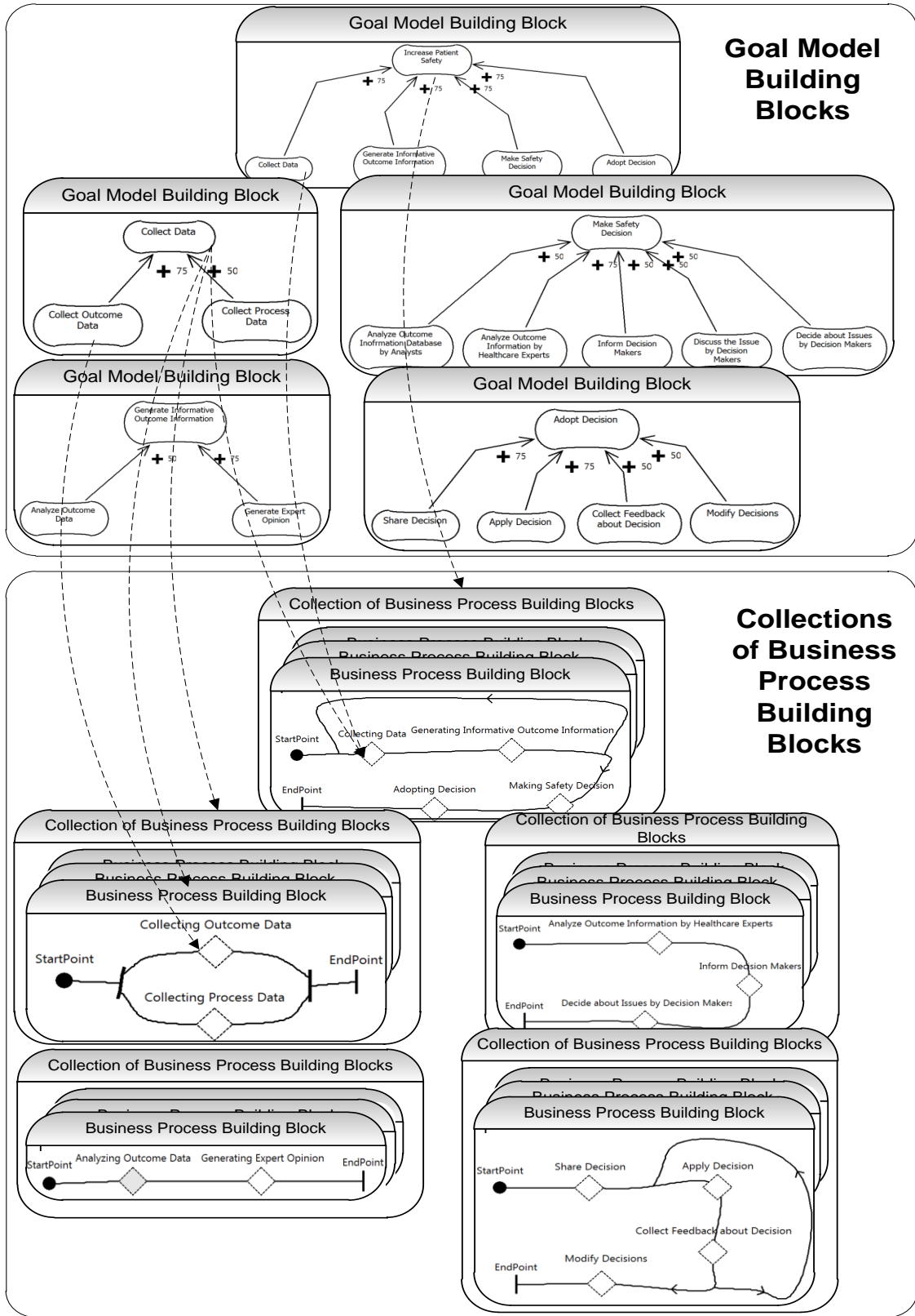
Figure 28 Collecting business process building blocks that address the problems in goal model building blocks
