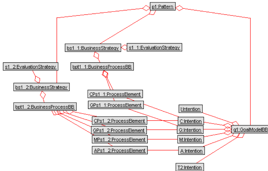
Figure 47 Object model of the p1 pattern after modification of its goal model building block
