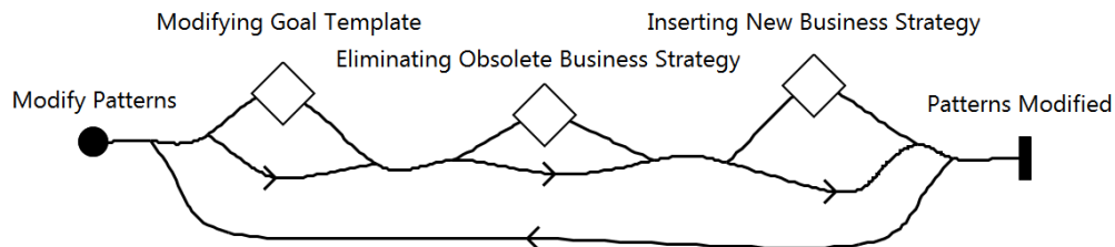
Figure 46 Main steps of the modification mechanism
