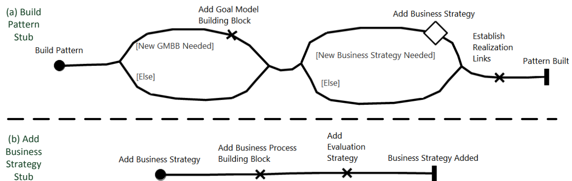
Figure 30 Forming a pattern using the components built when locating recurring problems and solutions
