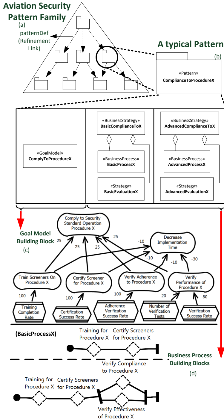
Figure 60 Artificial example : (a) Pattern family, (b) Pattern and its internal structure, (c) Goal model building block, (d) Business process building blocks
