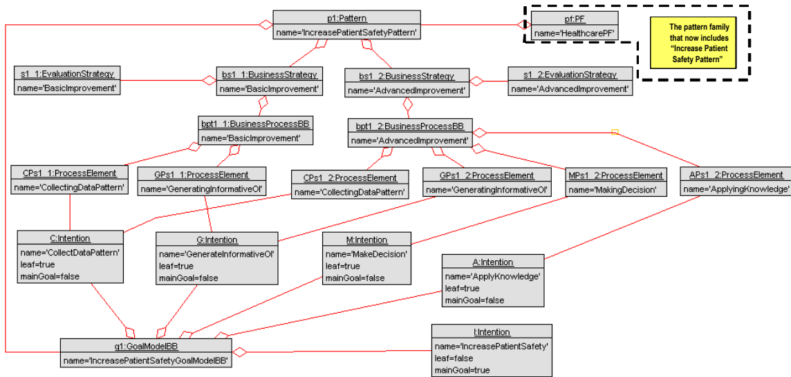
Figure 40 Object model of an empty PF extended to include Increase Patient Safety pattern
