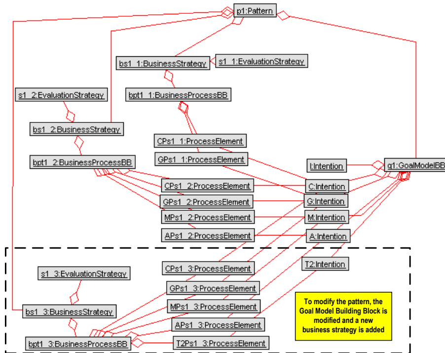
Figure 48 Object model of the p1 pattern after modification
