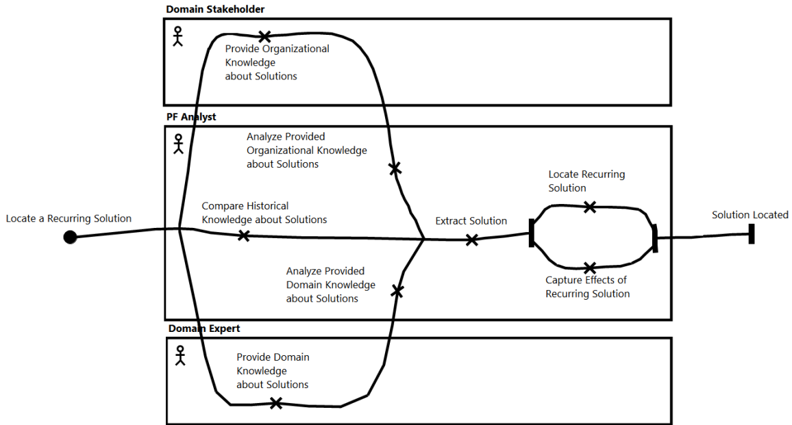
Figure 26 Locate a recurring solution in a particular domain
