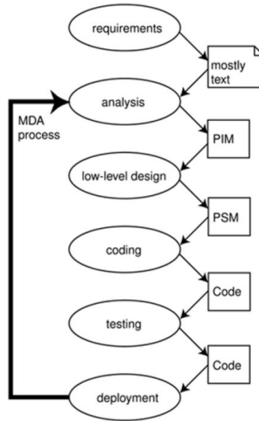
Figure 8 MDA software development life cycle [58]
