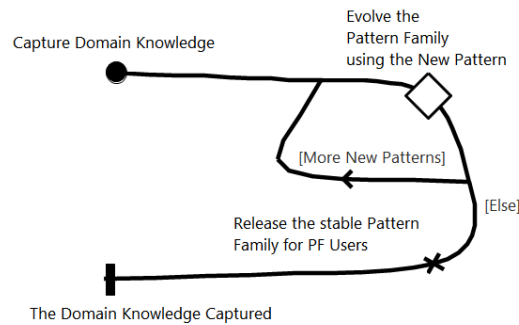
Figure 31 Add a newly built pattern to a pattern family
