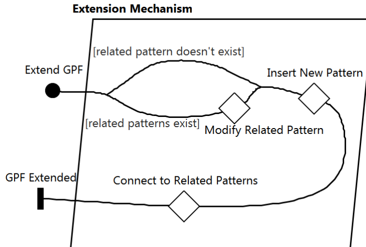
Figure 37 Main steps of the Extension Mechanism
