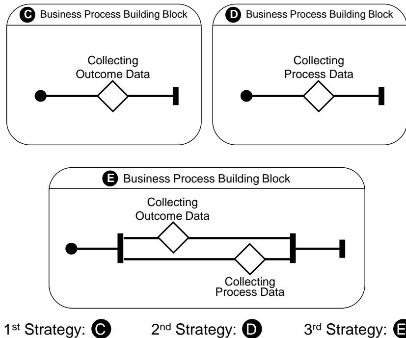
Figure 35 Business process building blocks for Collect Data
