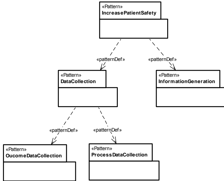
Figure 52 pf1 is a PF that contains patterns for ad-hoc approaches to improve patient safety
