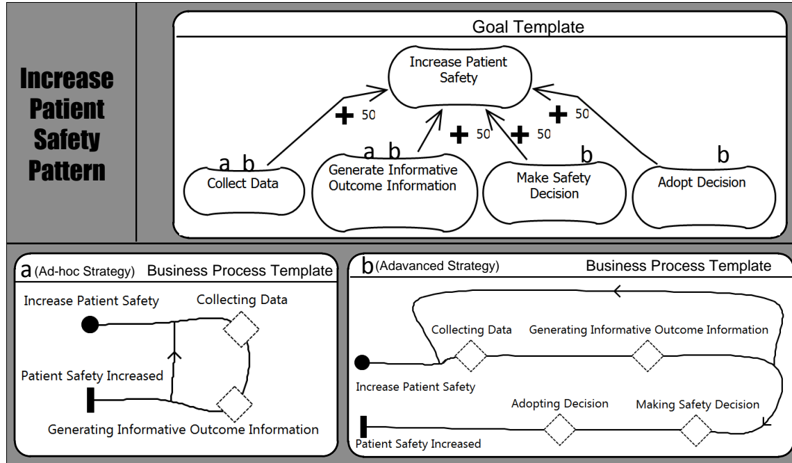
Figure 38 Top: goal model building block of xp - Bottom: business process building blocks of xp
