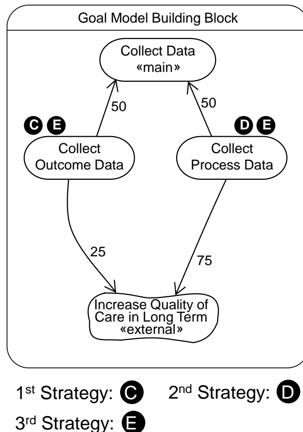
Figure 34 Goal model building block for Collect Data
