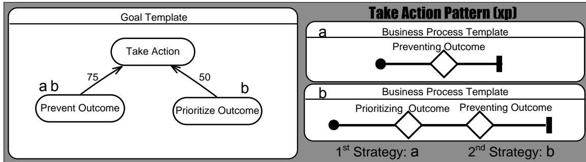
Figure 41 Left: goal model building block of xp - Right: business process building blocks of xp
