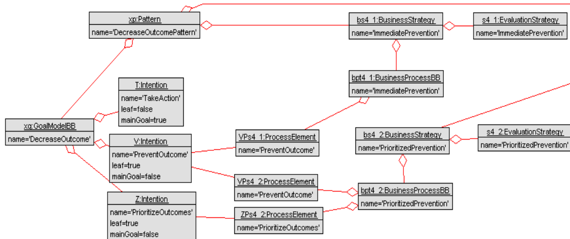
Figure 44 Object model of xp pattern
