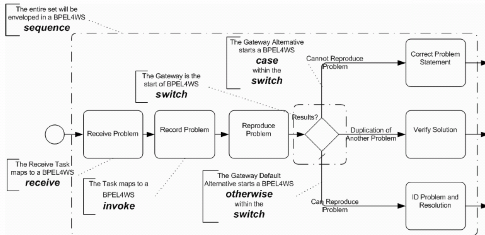
Figure 6 A BPMN model with annotation that shows mapping to BPEL4WS [48]
