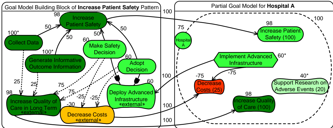
Figure 58 Using OCEM: linking goal model building blocks to the organizational goal model, with evaluations
