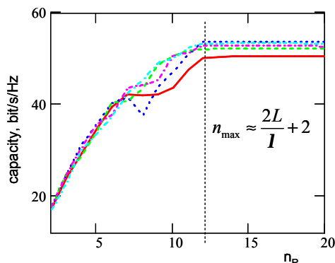
Fig. 1 MIMO channel capacity versus the number of antennas for L = 5\lambda .
